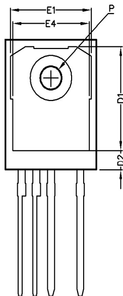
Bottom View
