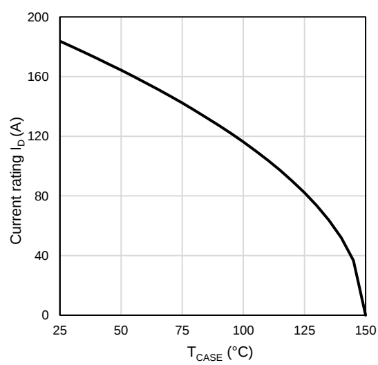
Figure 12: Current De-rating
