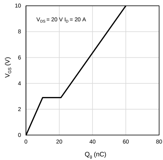
Figure 10: Gate-Charge Characteristics
