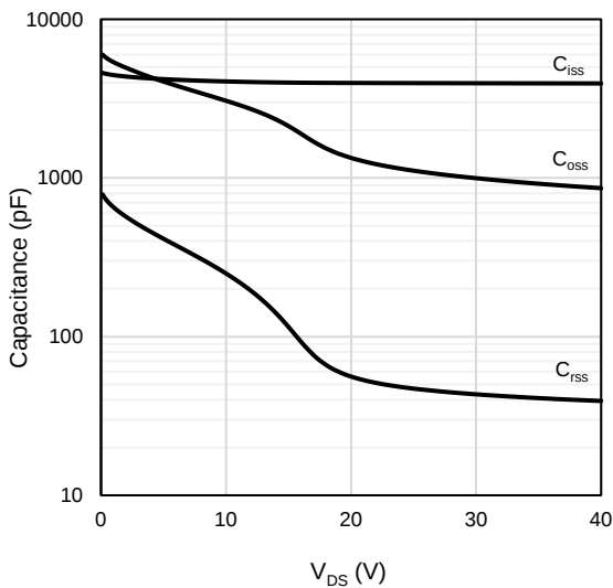
Figure 9: Capacitance Characteristics
