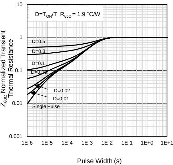
Figure 13: Normalized Maximum Transient Thermal Impedance
