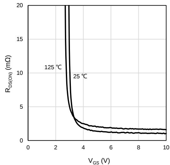
Figure 8: On-Resistance vs. Gate-Source Voltage
