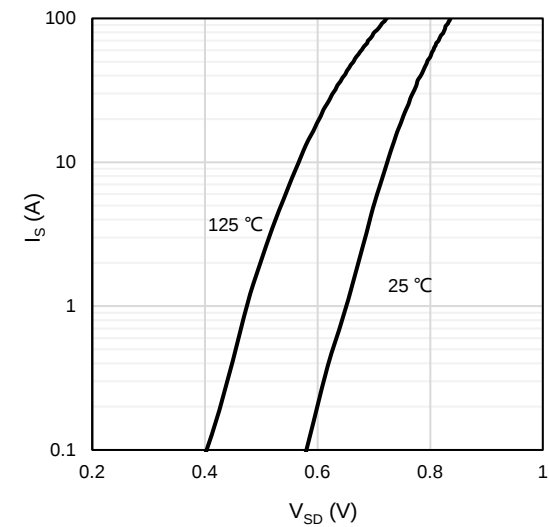
Figure 7: Body-Diode Characteristics
