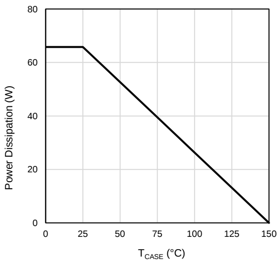
Figure 11: Power De-rating
