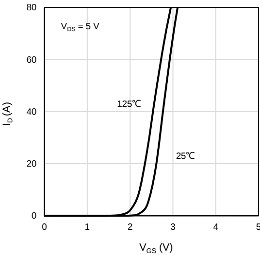
Figure 2: Transfer
