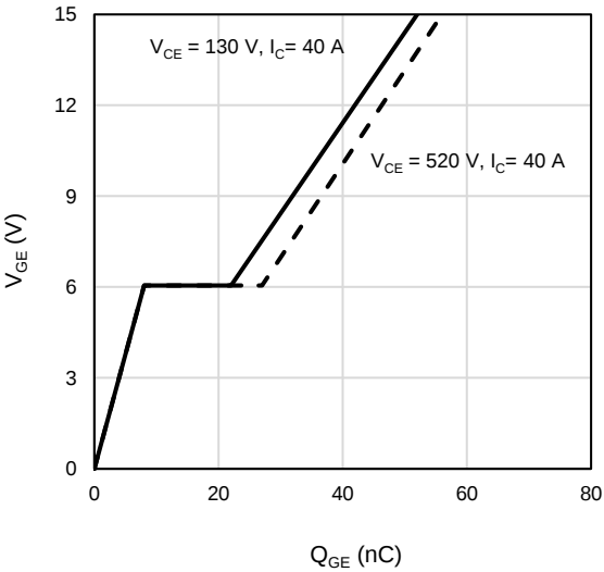
Figure 16: Gate-Charge Characteristics
