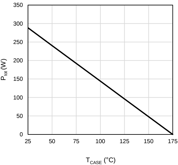
Figure 1: Power De-rating
